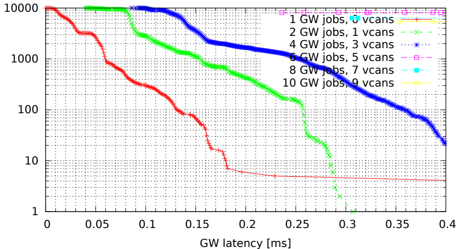
Chained GWs on multiple VCAN interfaces (GW kernel 2.6.33.7-00007-g9c0ff90, Traffic flood, Load cpu)
