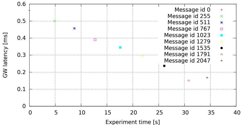
2048 GW rules (one per id, mask 0x7FF), no modifications (GW kernel 2.6.33.7-00007-g9c0ff90, Traffic flood, Load cpu)
