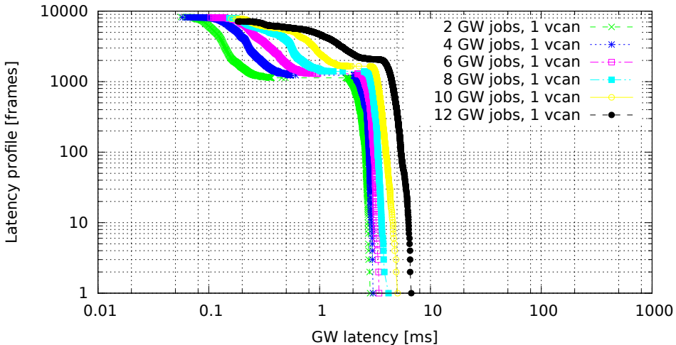
Chained GWs on a single VCAN interface (GW kernel 2.6.33.7-00007-g9c0ff90, Traffic 50, Load eth)
