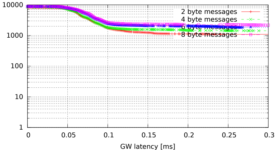
Single GW rule for all messages, no modifications (GW kernel 2.6.33.7-00007-g9c0ff90, Traffic 50, Load eth)
