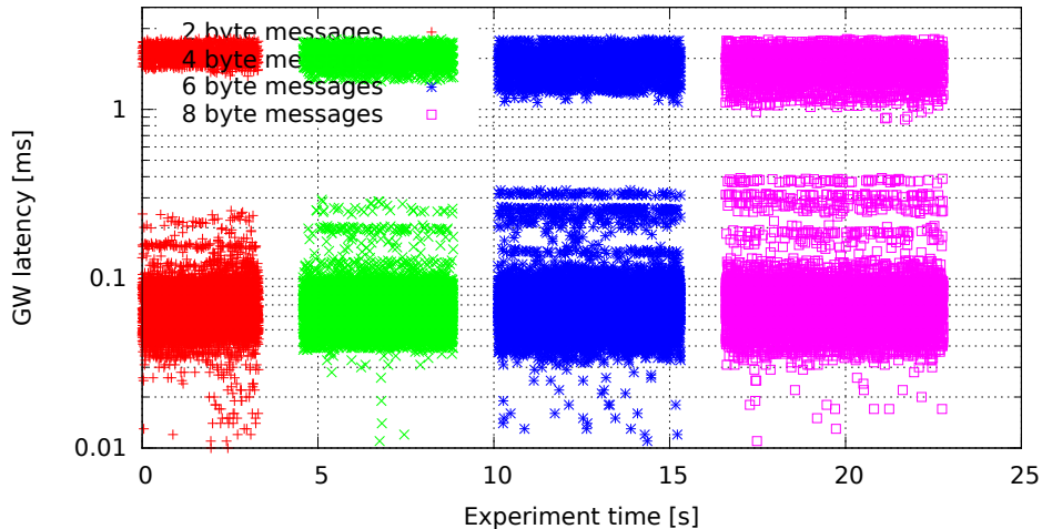
Single GW rule for all messages, no modifications, high (soft)irq task priority (GW kernel 2.6.33.7-00007-g9c0ff90, Traffic 50, Load eth)
