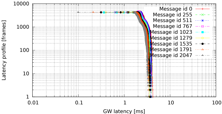
2048 GW rules (one per id, mask 0x7FF), no modifications (GW kernel 2.6.33.7-00007-g9c0ff90, Traffic 50, Load eth)
