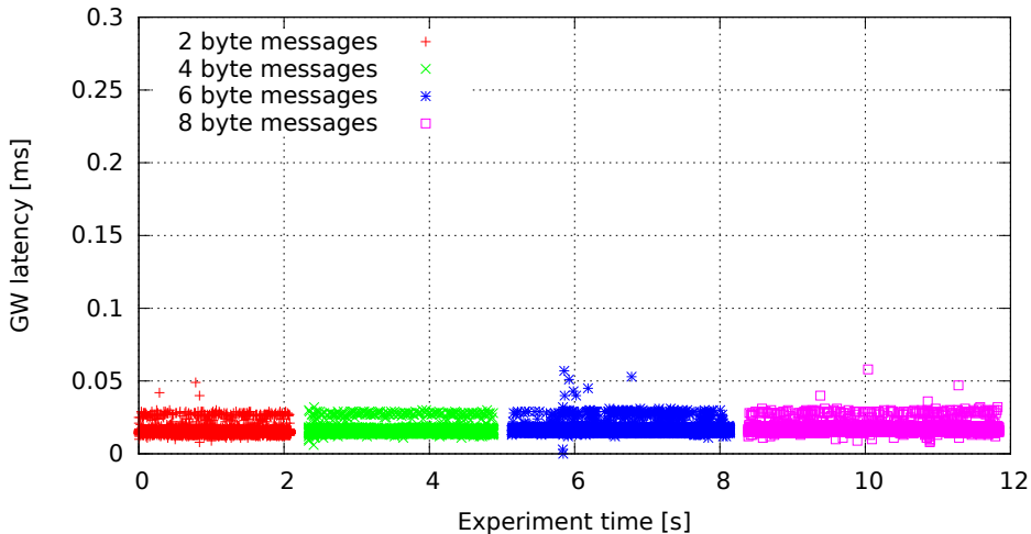
Single GW rule for all messages, no modifications (GW kernel rtems4.10-midam, Traffic oneatatime, Load none)
