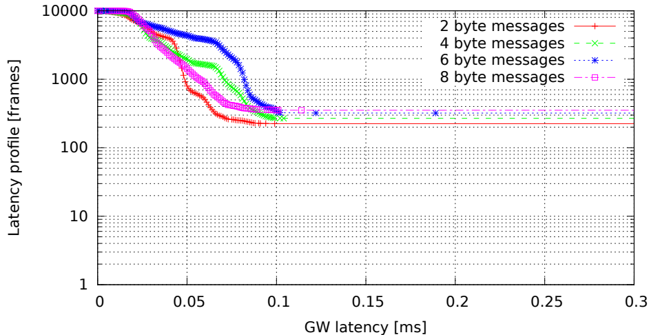
Single GW rule for all messages, no modifications (GW kernel rtems4.10-midam, Traffic oneatatime, Load eth)
