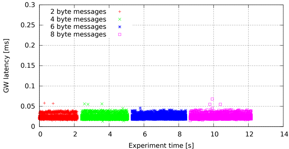
Single GW rule for all messages, no modifications (GW kernel rtems4.10-midam, Traffic oneatatime, Load cpu)
