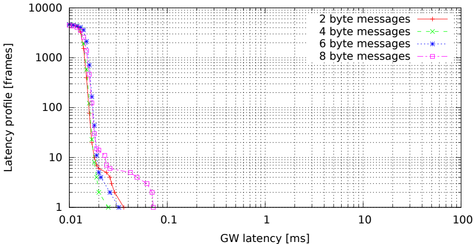
Single GW rule for all messages, no modifications, high (soft)irq task priority (GW kernel rtems4.10-midam, Traffic flood, Load none)
