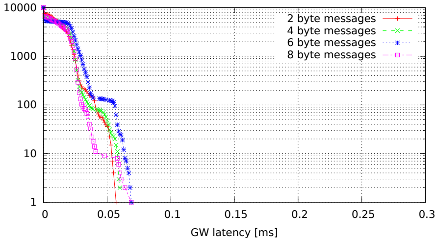
Single GW rule for all messages, no modifications (GW kernel rtems4.10-midam, Traffic flood, Load cpu)
