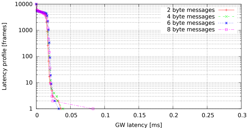
Single GW rule for all messages, no modifications, high (soft)irq task priority (GW kernel rtems4.10-midam, Traffic flood, Load cpu)
