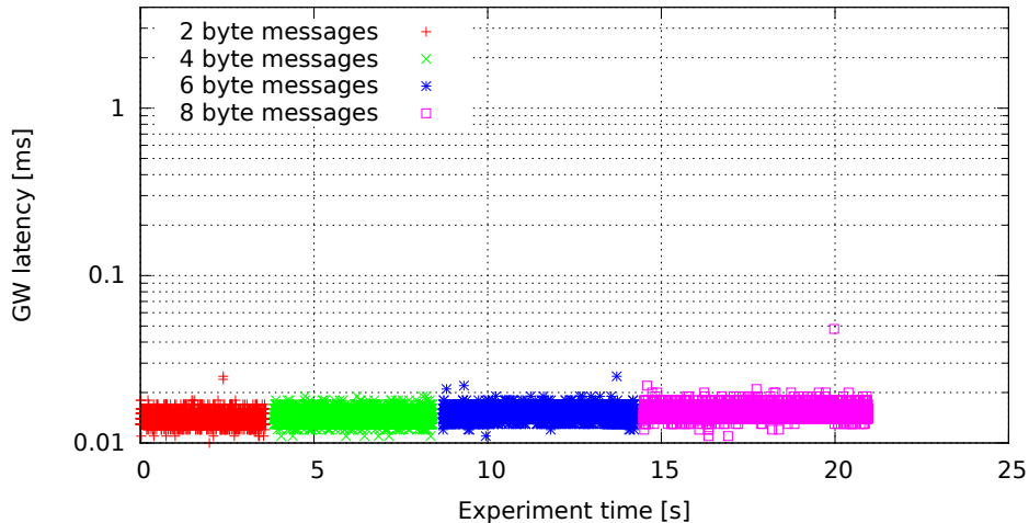
Single GW rule for all messages, no modifications, high (soft)irq task priority (GW kernel rtems4.10-midam, Traffic 50, Load none)
