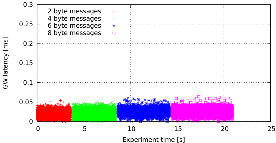
Single GW rule for all messages, no modifications, high (soft)irq task priority (GW kernel rtems4.10-midam, Traffic 50, Load eth)
