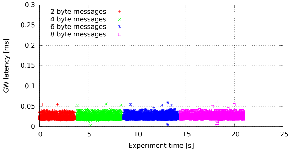
Single GW rule for all messages, no modifications (GW kernel rtems4.10-midam, Traffic 50, Load cpu)
