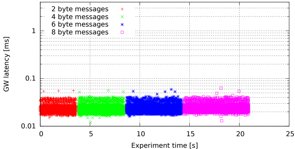
Single GW rule for all messages, no modifications (GW kernel rtems4.10-midam, Traffic 50, Load cpu)
