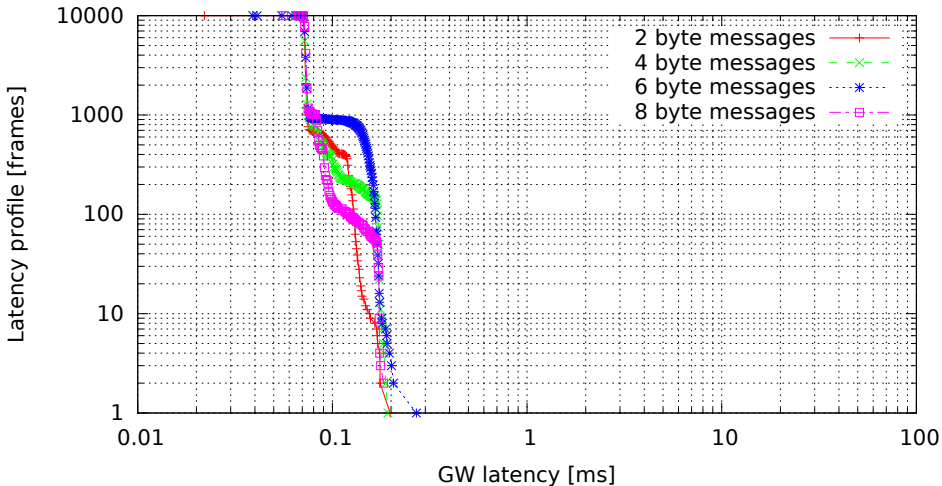
Single GW rule for all messages, no modifications (GW kernel 3.4.33-rt47-00004-gc58c9ae, Traffic oneatatime, Load none)
