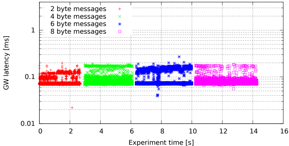
Single GW rule for all messages, no modifications (GW kernel 3.4.33-rt47-00004-gc58c9ae, Traffic oneatatime, Load none)
