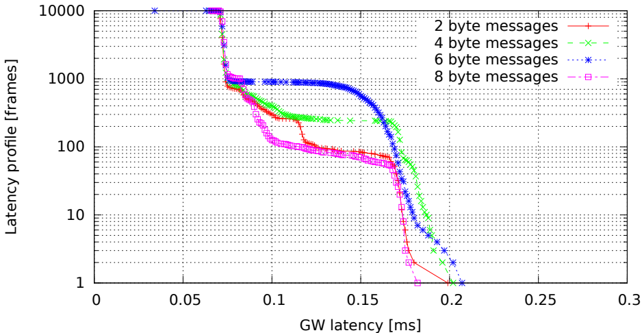
Single GW rule for all messages, no modifications, high (soft)irq task priority (GW kernel 3.4.33-rt47-00004-gc58c9ae, Traffic oneatatime, Load none)
