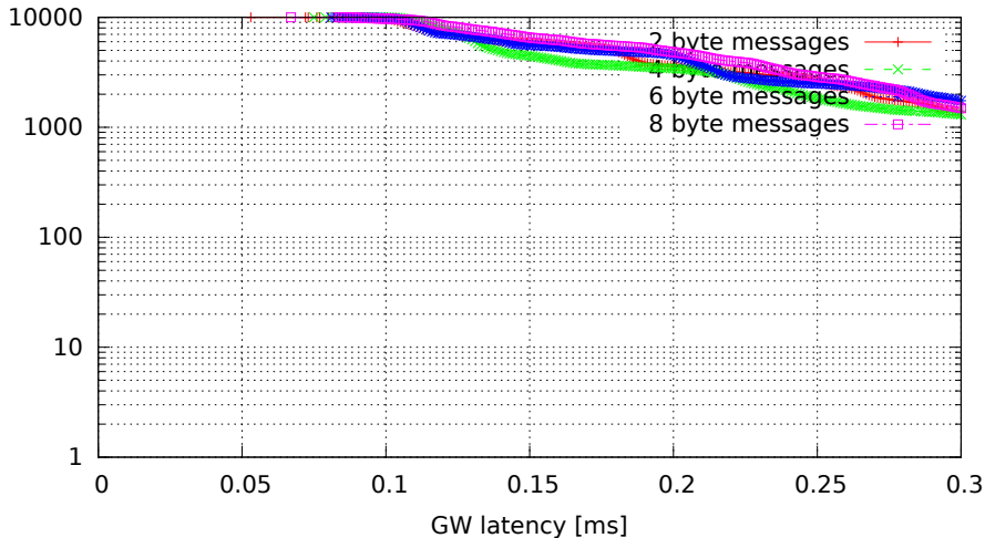
Single GW rule for all messages, no modifications (GW kernel 3.4.33-rt47-00004-gc58c9ae, Traffic onetotime, Load eth)
