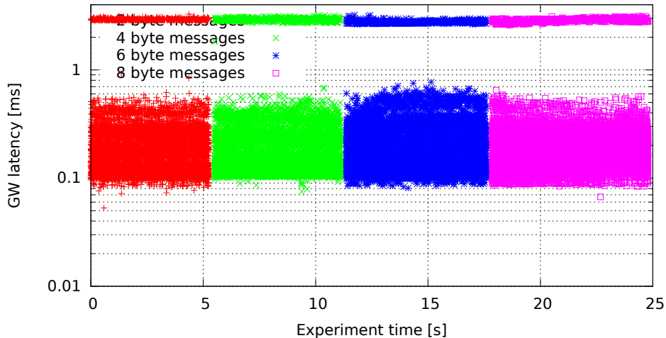
Single GW rule for all messages, no modifications (GW kernel 3.4.33-rt47-00004-gc58c9ae, Traffic onetotime, Load eth)
