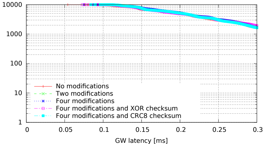
Single GW rule for all messages with modifications, 8 byte messages (GW kernel 3.4.33-rt47-00004-gc58c9ae, Traffic onetotime, Load eth)
