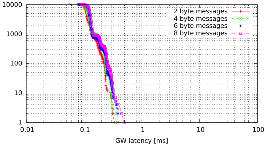
Single GW rule for all messages, no modifications (GW kernel 3.4.33-rt47-00004-gc58c9ae, Traffic oneatatime, Load cpu)
