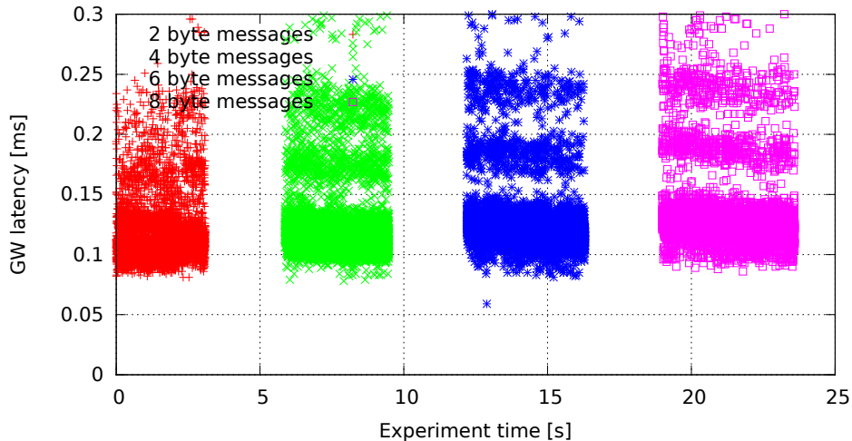
Single GW rule for all messages, no modifications (GW kernel 3.4.33-rt47-00004-gc58c9ae, Traffic oneatatime, Load cpu)
