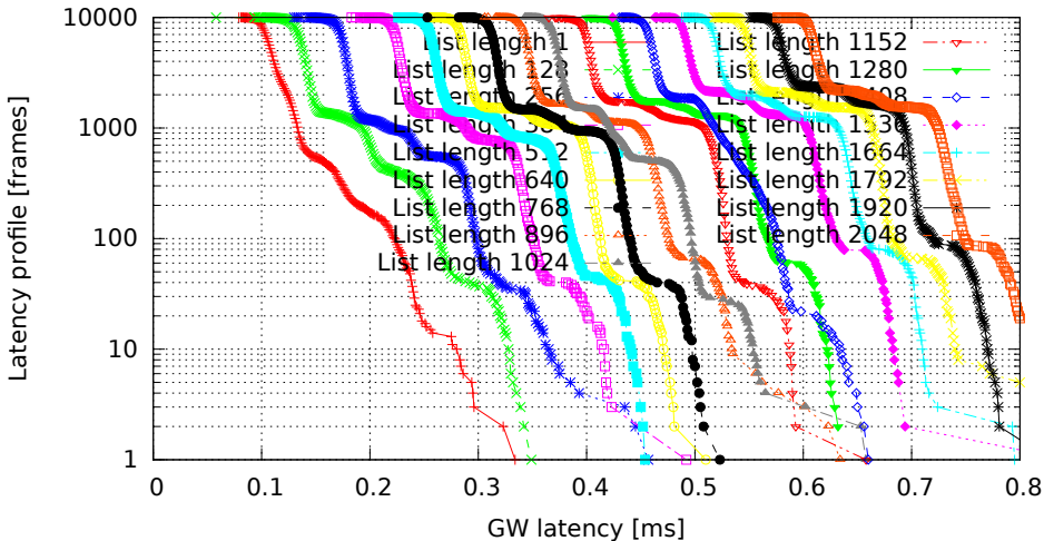
Different lengths of filter list, only the last one matches (GW kernel 3.4.33-rt47-00004-gc58c9ae, Traffic oneatime, Load cpu)
