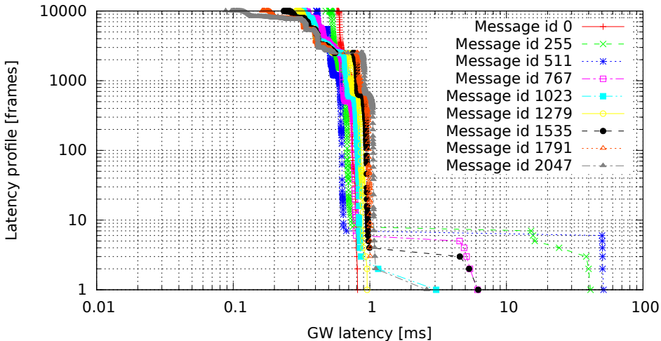
2048 GW rules (one per id, mask 0x7FF), no modifications (GW kernel 3.4.33-rt47-00004-gc58c9ae, Traffic onetatime, Load cpu)
