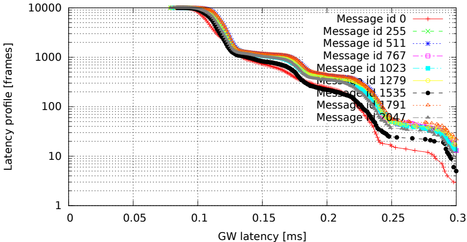
2048 GW rules (one per id, mask C00007FF), no modifications (GW kernel 3.4.33-rt47-00004-gc58c9ae, Traffic oneatatime, Load cpu)
