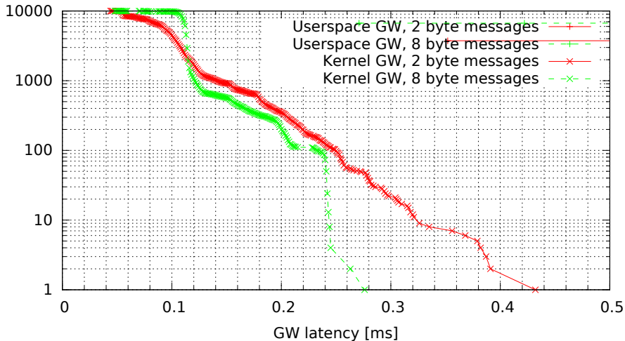
Kernel vs. userspace GW, no modifications (GW kernel 3.4.33-rt47-00004-gc58c9ae, Traffic flood, Load none)
