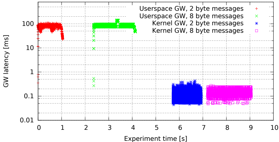
Single GW rule for all messages, no modifications (GW kernel 3.4.33-rt47-00004-gc58c9ae, Traffic flood, Load none)
