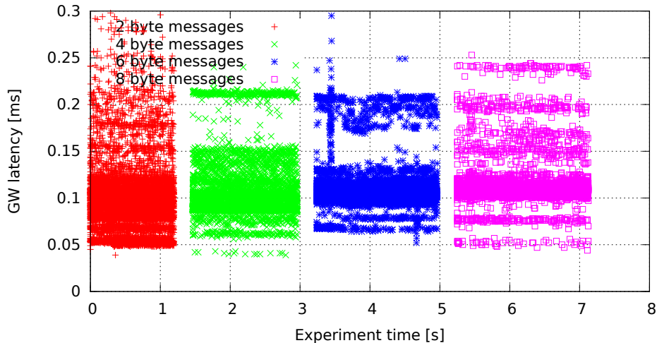
Single GW rule for all messages, no modifications (GW kernel 3.4.33-rt47-00004-gc58c9ae, Traffic flood, Load none)
