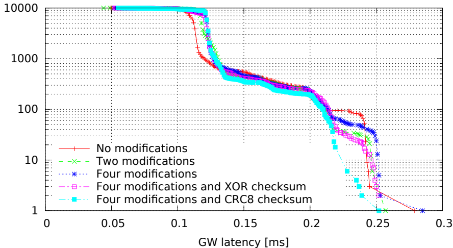
Single GW rule for all messages with modifications, 8 byte messages (GW kernel 3.4.33-rt47-00004-gc58c9ae, Traffic flood, Load none)
