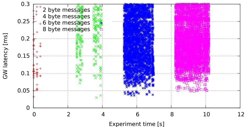
Single GW rule for all messages, no modifications (GW kernel 3.4.33-rt47-00004-gc58c9ae, Traffic flood, Load eth)
