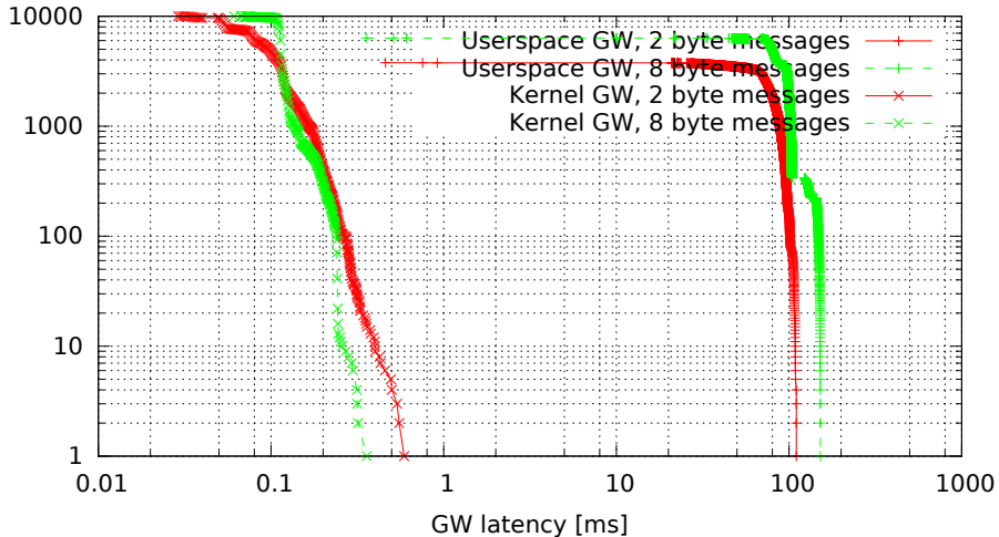
Kernel vs. userspace GW, no modifications (GW kernel 3.4.33-rt47-00004-gc58c9ae, Traffic flood, Load cpu)
