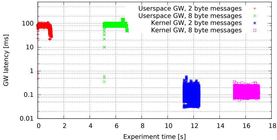
Single GW rule for all messages, no modifications (GW kernel 3.4.33-rt47-00004-gc58c9ae, Traffic flood, Load cpu)
