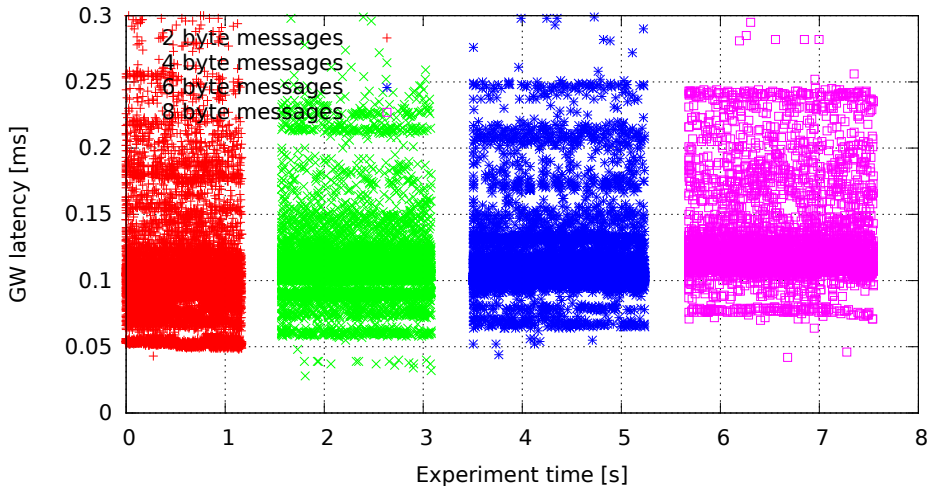
Single GW rule for all messages, no modifications, high (soft)irq task priority (GW kernel 3.4.33-rt47-00004-gc58c9ae, Traffic flood, Load cpu)
