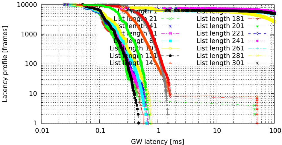
Different lengths of filter list, only the last one matches (GW kernel 3.4.33-rt47-00004-gc58c9ae, Traffic flood, Load cpu)
