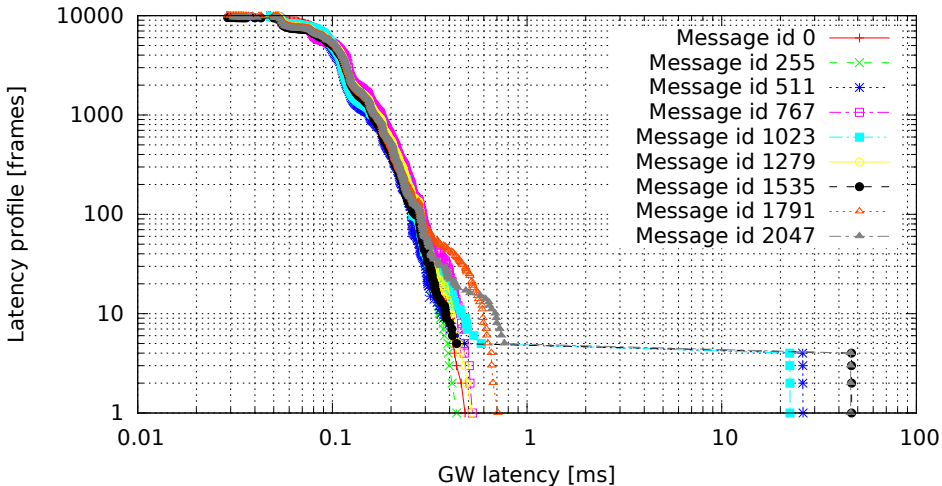
2048 GW rules (one per id, mask C00007FF), no modifications (GW kernel 3.4.33-rt47-00004-gc58c9ae, Traffic flood, Load cpu)
