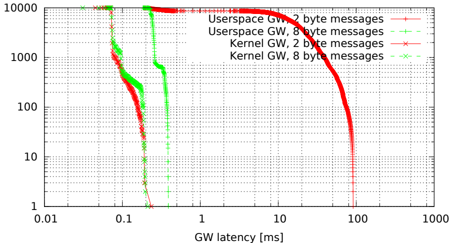
Kernel vs. userspace GW, no modifications (GW kernel 3.4.33-rt47-00004-gc58c9ae, Traffic 50, Load none)
