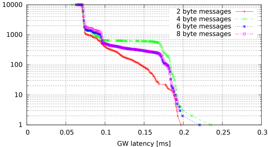
Single GW rule for all messages, no modifications, high (soft)irq task priority (GW kernel 3.4.33-rt47-00004-gc58c9ae, Traffic 50, Load none)
