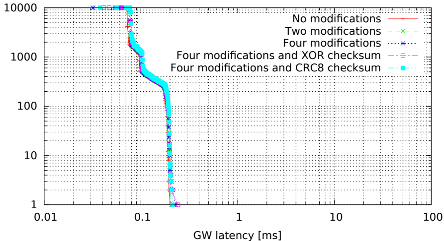
Single GW rule for all messages with modifications, 8 byte messages (GW kernel 3.4.33-rt47-00004-gc58c9ae, Traffic 50, Load none)
