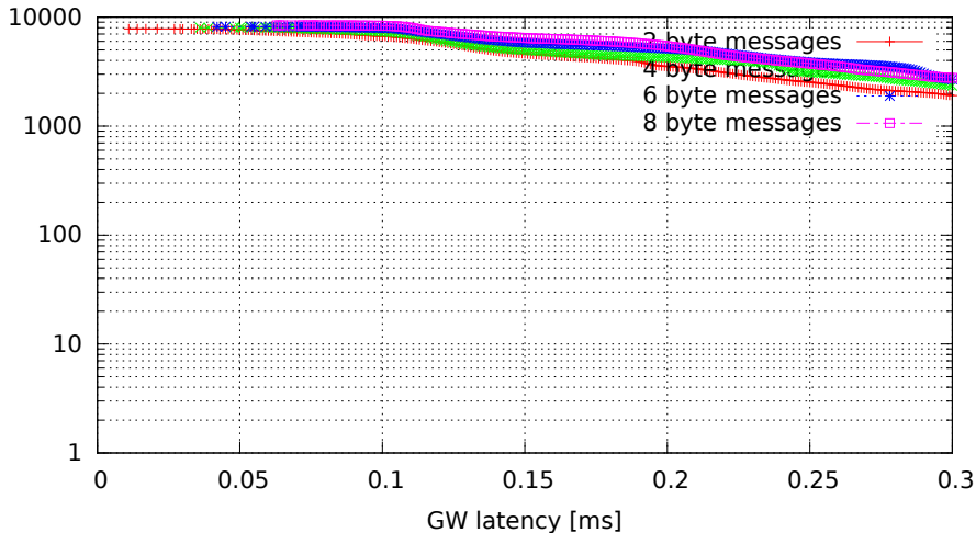
Single GW rule for all messages, no modifications (GW kernel 3.4.33-rt47-00004-gc58c9ae, Traffic 50, Load eth)
