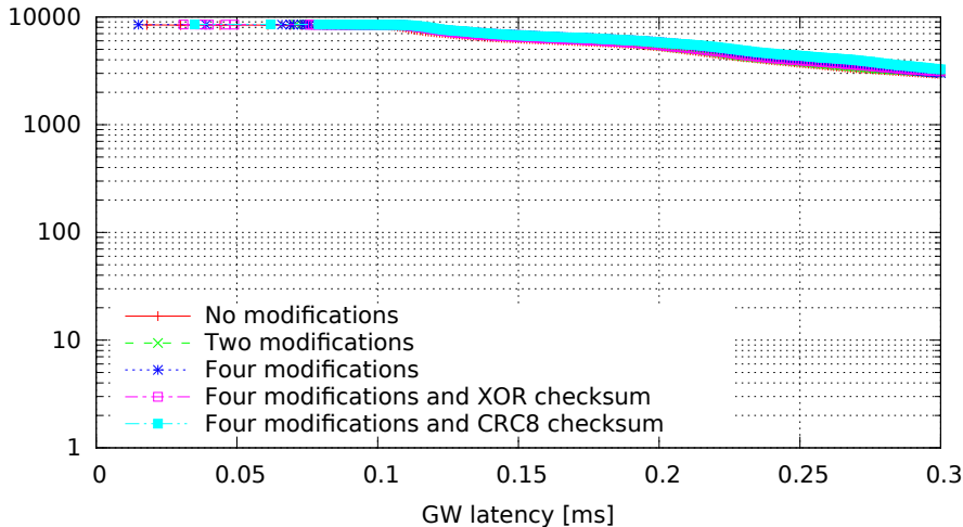
Single GW rule for all messages with modifications, 8 byte messages (GW kernel 3.4.33-rt47-00004-gc58c9ae, Traffic 50, Load eth)
