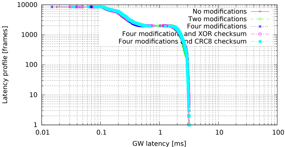
Single GW rule for all messages with modifications, 8 byte messages (GW kernel 3.4.33-rt47-00004-gc58c9ae, Traffic 50, Load eth)
