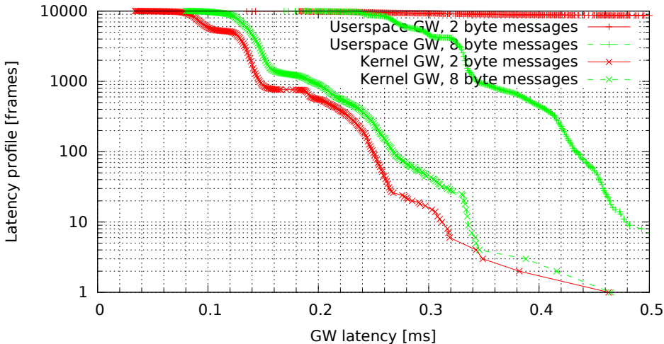
Kernel vs. userspace GW, no modifications (GW kernel 3.4.33-rt47-00004-gc58c9ae, Traffic 50, Load cpu)
