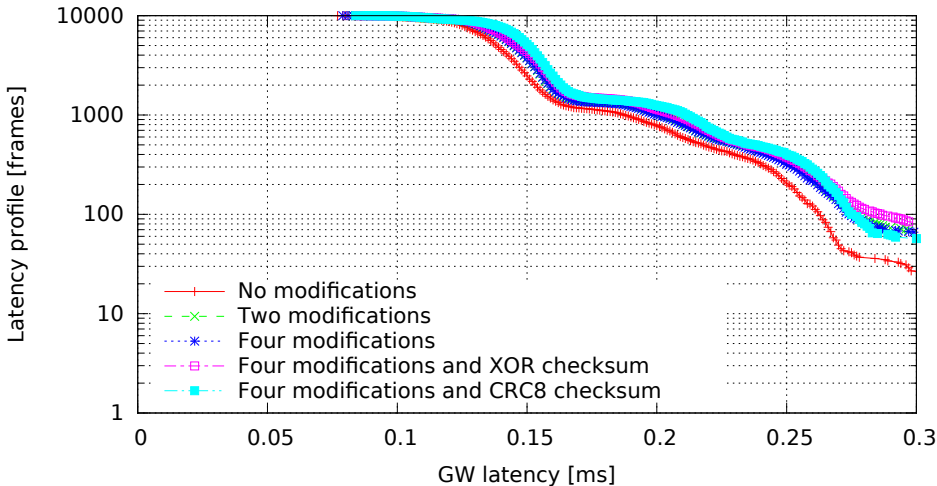
Single GW rule for all messages with modifications, 8 byte messages (GW kernel 3.4.33-rt47-00004-gc58c9ae, Traffic 50, Load cpu)
