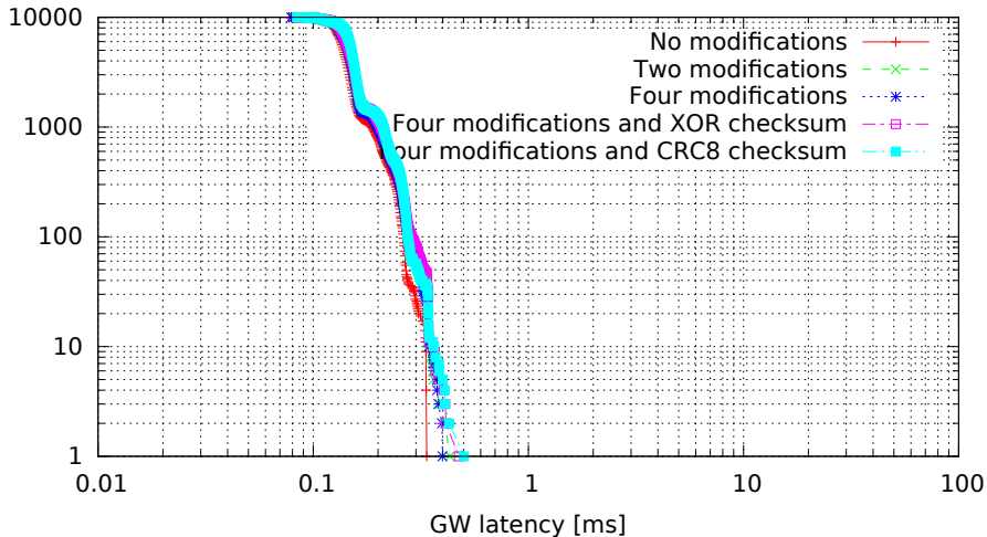
Single GW rule for all messages with modifications, 8 byte messages (GW kernel 3.4.33-rt47-00004-gc58c9ae, Traffic 50, Load cpu)
