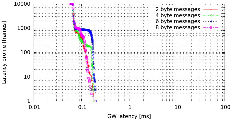
Single GW rule for all messages, no modifications (GW kernel 3.0.7-rt20-00008-g0c18035, Traffic oneatatime, Load none)
