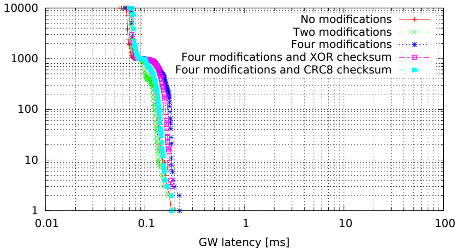
Single GW rule for all messages with modifications, 8 byte messages (GW kernel 3.0.7-rt20-00008-g0c18035, Traffic oneatatime, Load none)
