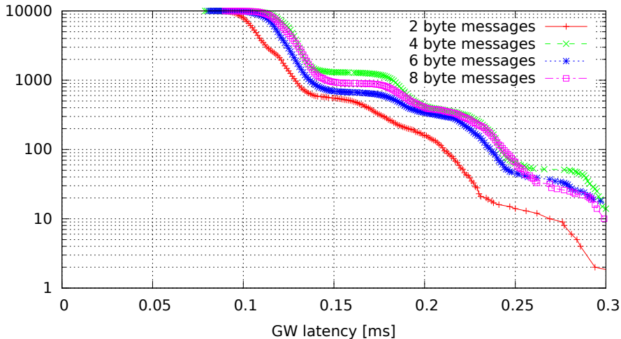
Single GW rule for all messages, no modifications (GW kernel 3.0.7-rt20-00008-g0c18035, Traffic oneatatime, Load cpu)
