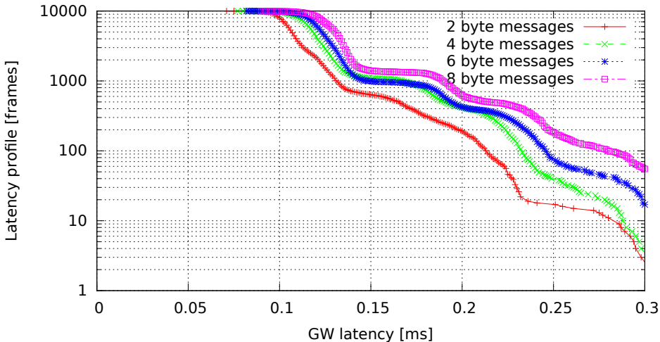
Single GW rule for all messages, no modifications, high (soft)irq task priority (GW kernel 3.0.7-rt20-00008-g0c18035, Traffic onetime, Load cpu)
